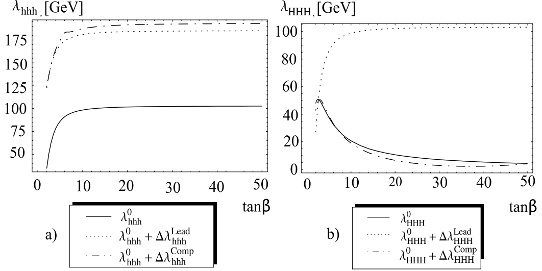
Fig.3: Dependence of the trilinear Higgs self-couplings (on the tree and one-loop levels) on \tan\beta , for \sqrt{s} = m_{H_{g1}} + m_{H_{g2}} + 10 GeV, M_A = 500 GeV, M_3 = \mu = 300 GeV, M_{\tilde{Q}} = M_{\tilde{U}} = M_{\tilde{D}} = M_{\tilde{R}} = M_{\tilde{L}} = 1 TeV, A_f = 200 GeV.
