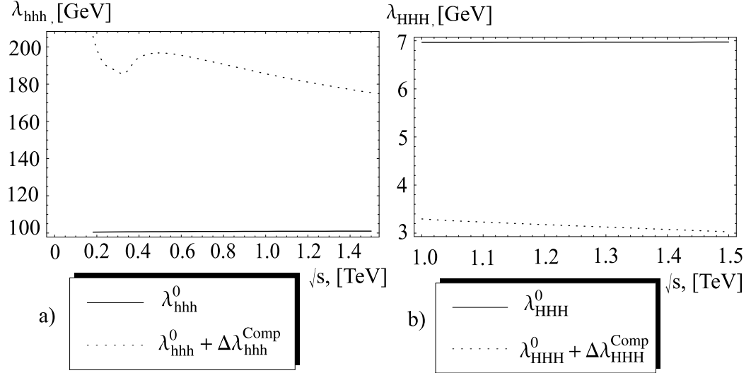
Fig.4: Dependence of the trilinear Higgs self-couplings (on the tree and one-loop levels) on \sqrt{s} , for \tan\beta = 30 , M_A = 500 GeV, M_3 = \mu = 300 GeV, M_{\tilde{Q}} = M_{\tilde{U}} = M_{\tilde{D}} = M_{\tilde{R}} = M_{\tilde{L}} = 1 TeV, A_f = 200 GeV.
