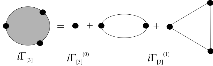
Fig.2: Vertex function decomposition: the one-loop approximation.
