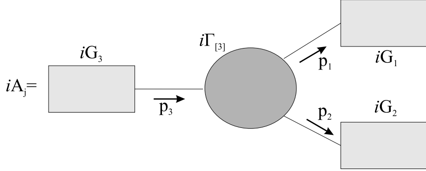
Fig.1: Feynman diagram for amplitude A_j .
